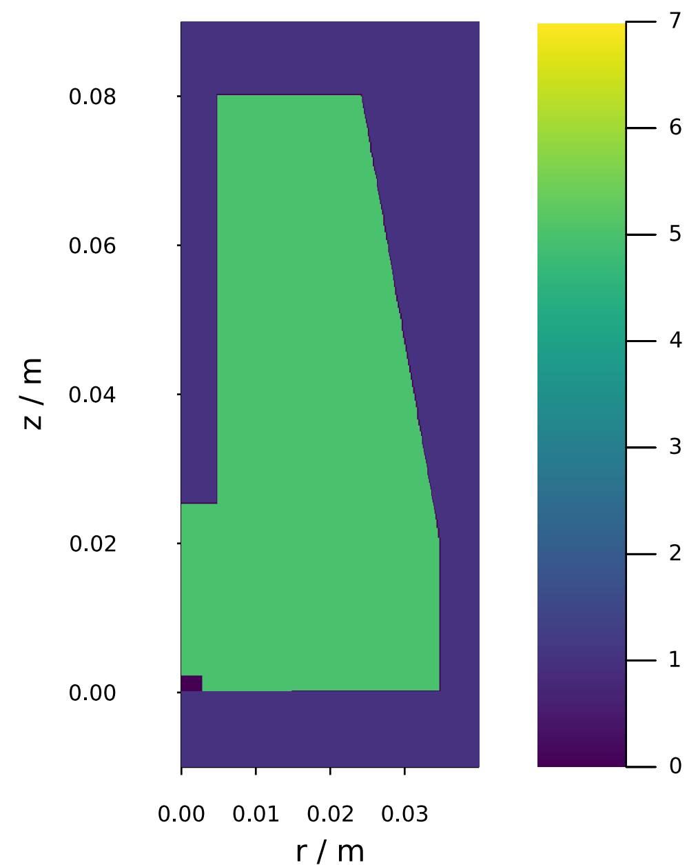
Point Type Map @ \varphi = 0.0^\circ
