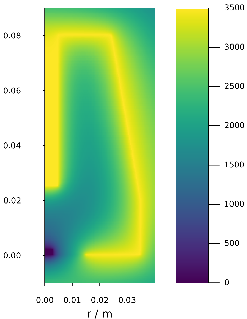
Electric Potential @ \varphi = 20.0^\circ
