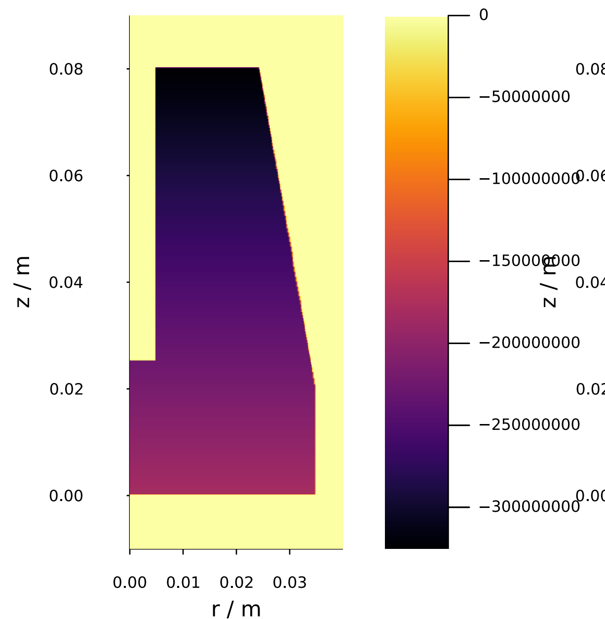
Effective Charge Density @ \varphi = 0.0^\circ
