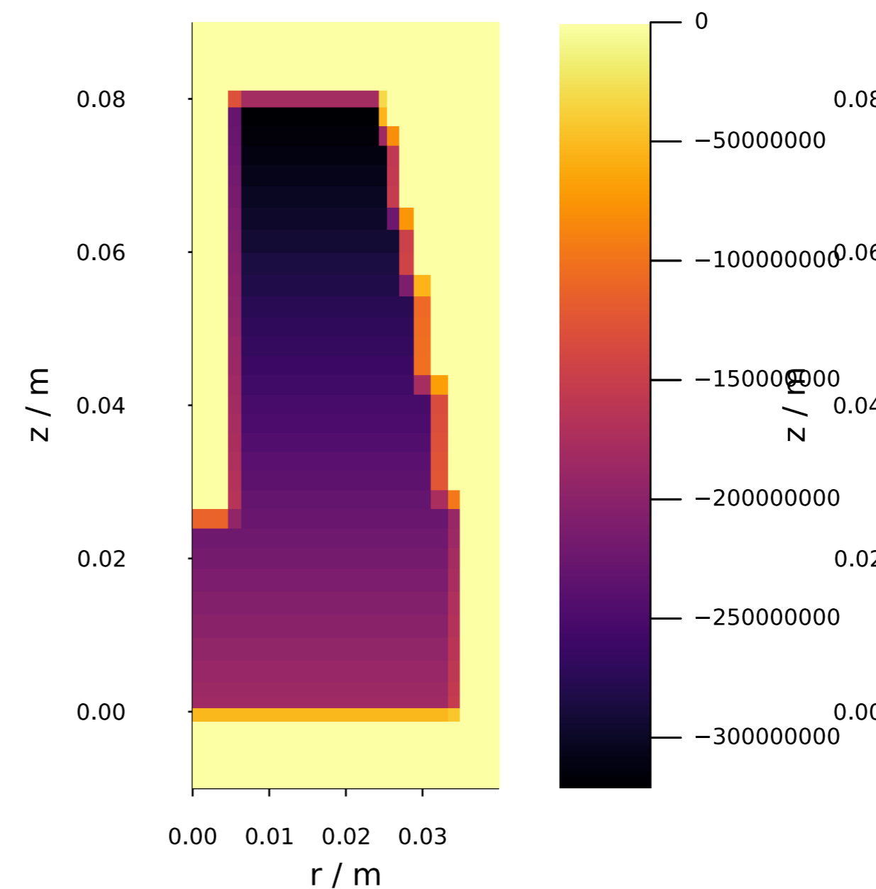
Effective Charge Density @ \varphi = 0.0^\circ
