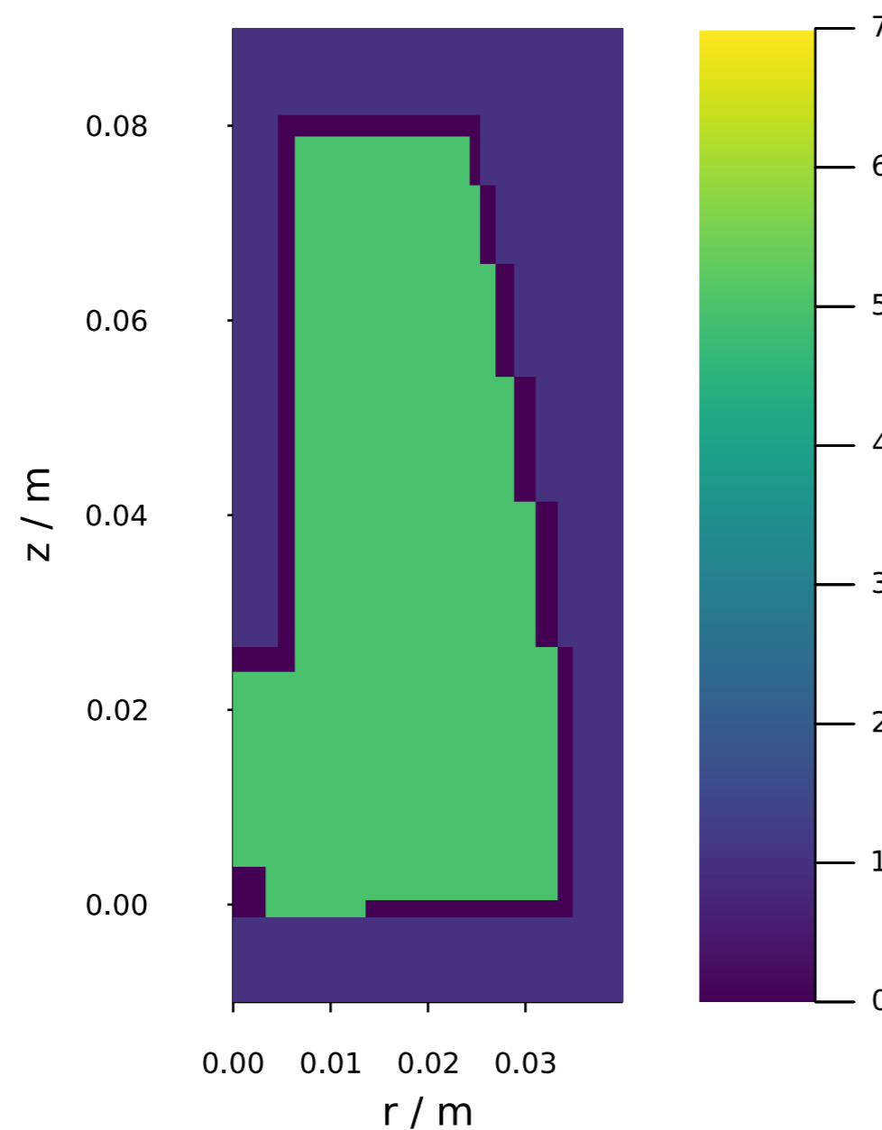
Point Type Map @ \varphi = 0.0^\circ
