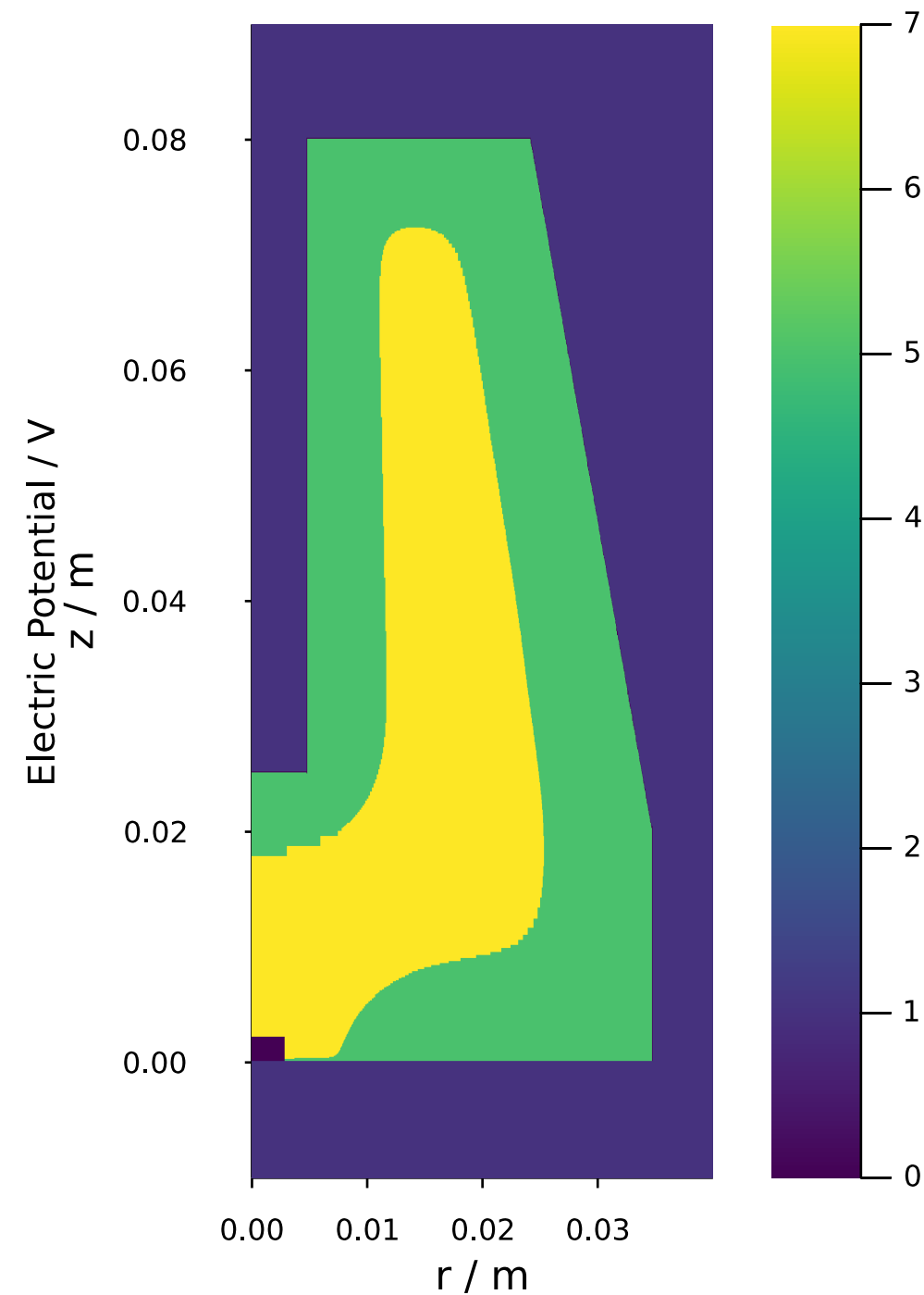
Point Type Map @ \varphi = 0.0^\circ
