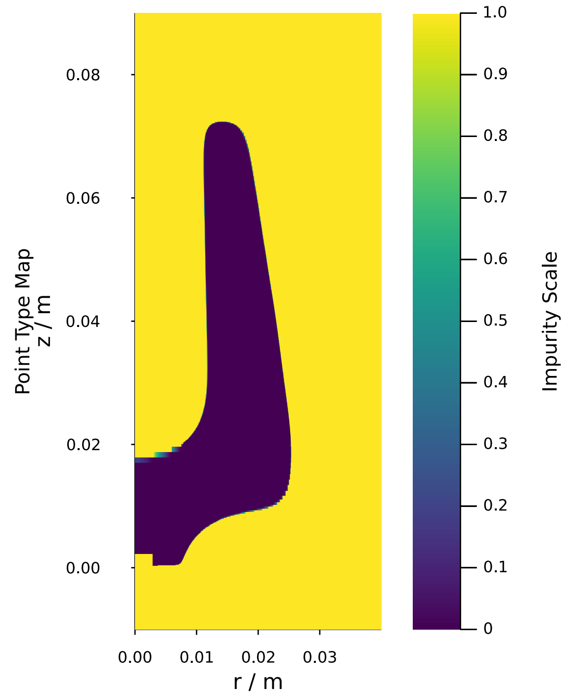
Impurity Scale @ \varphi = 0.0^\circ
