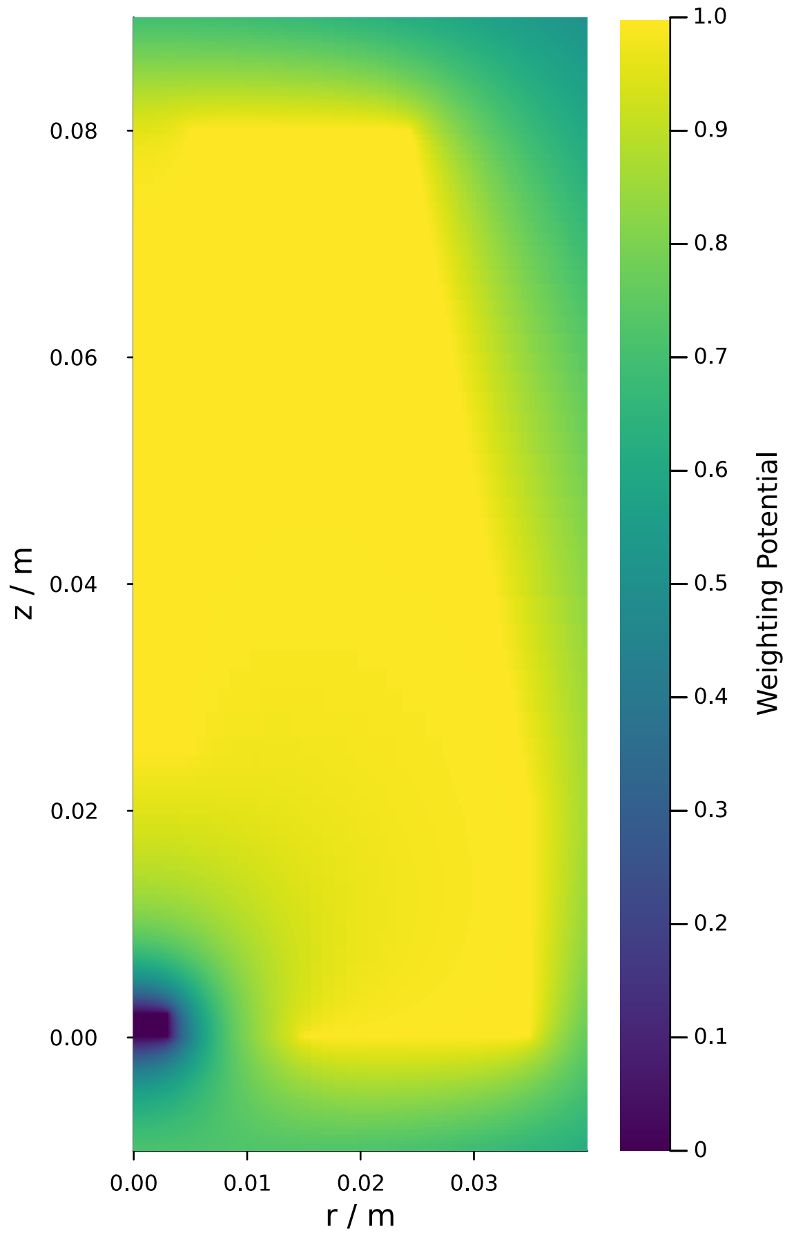
Weighting Potential @ \phi = 0.0^\circ
