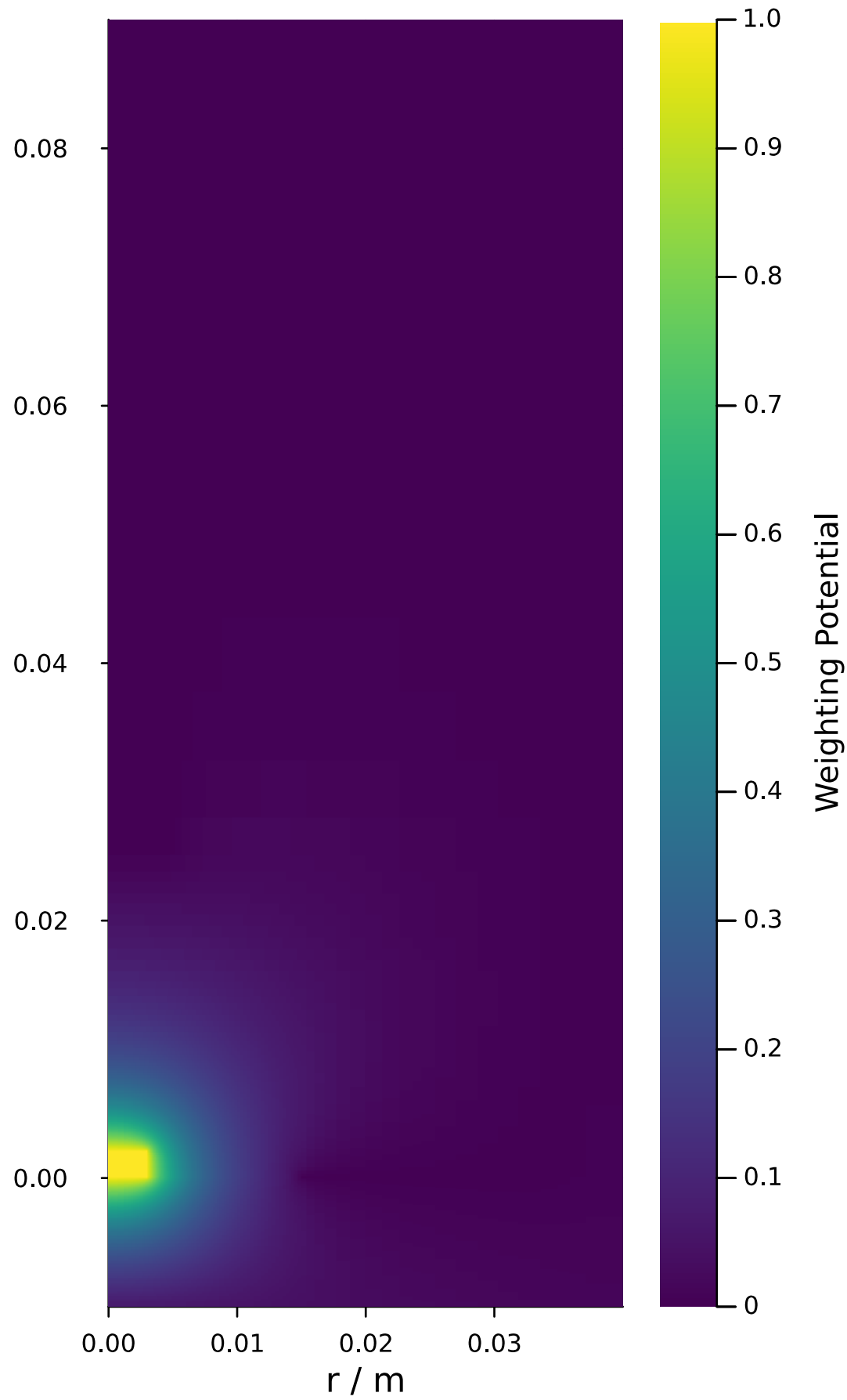
Weighting Potential @ \phi = 0.0^\circ
